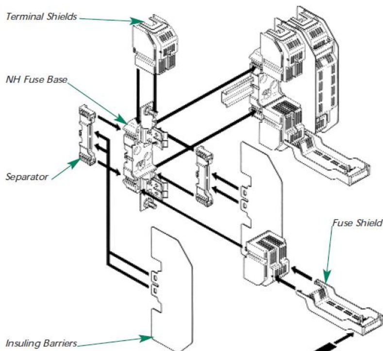
Typical NH Polyester Fuse Base Assembly - Exploded View
