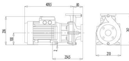
Electro motor - CM40D140EM2M50
