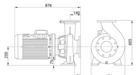
Electro motor - CM125D250EM4T50
