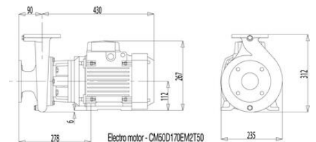
Electro motor - CM50D170EM2T50
