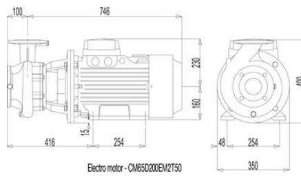
Electro motor - CM6SD200EM2T50
