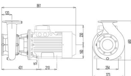
Electro motor - CM100D155EM2T50
