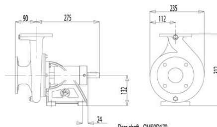
Bare shaft - CM50D170
