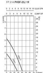
Performance charts*
