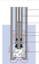
F 310 - The small drum pump with mechanical seal
