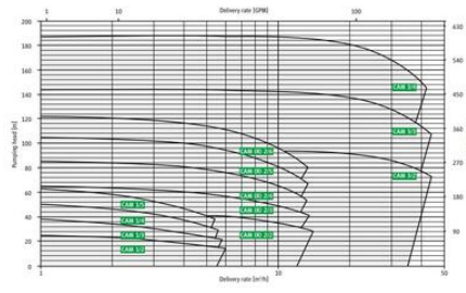
3500 rpm 60 Hz
