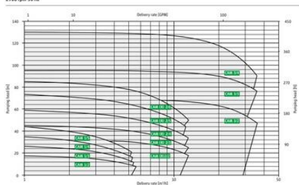
CHARACTERISTIC MAPS
