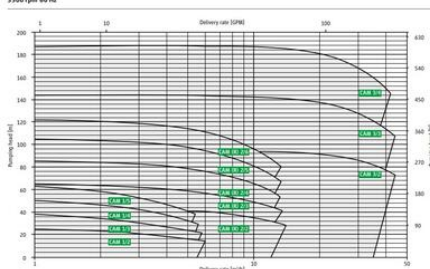
CHARACTERISTIC MAPS
