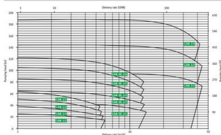
CHARACTERISTIC MAPS
