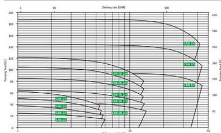
CHARACTERISTIC MAPS
