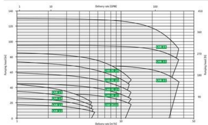
CHARACTERISTIC MAPS
