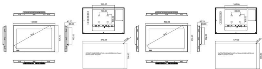
Panel Cut-out Dimensions: 479.30 x 300.30 mm (18.87" x 11.82")
