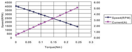
MB054TP100 CURVE
