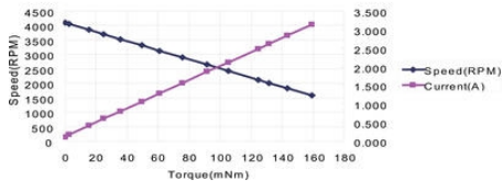
MB042DK200 CURVE
