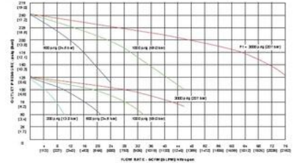
C v = 0.06 Model Metal Diaphragm
