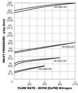
44-2300 Typical Application
