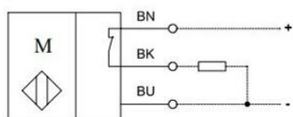
Wiring diagram
