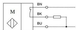
Wiring diagram
