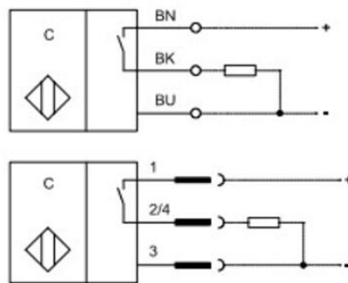
PNP – Proximity Switch
