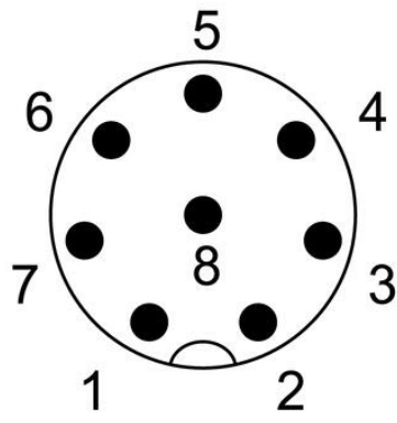
M12 8-pole connector
