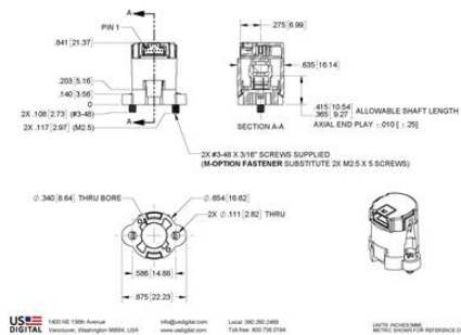
M3K Magnetic Kit Encoder (5-Option Bolt Circle)
