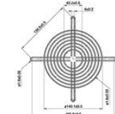
MG-16 (For UF16FC Series) *Steel
