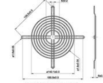
MG-25 (For UF25HC, 25GC, 25GCA, 25GCB, 20JC Series) *Steel
