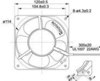
Terminal or Lead Wire Type
