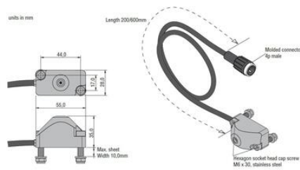
Front side 4p molded male connector
