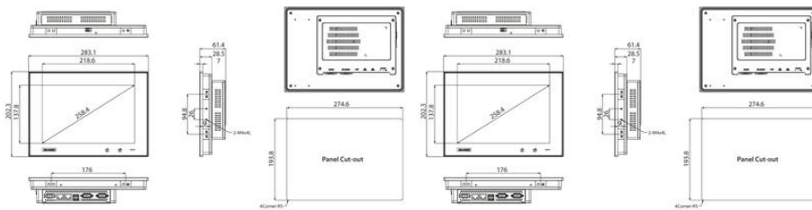
TPC-1051WP Panel Cut-out Dimensions: 274.6 x 193.8 mm
